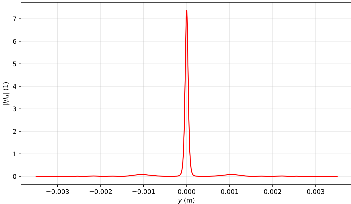
Intensity profile I(x=0, y, z=0.796)/I_0 , P_{in}=7.0P_{cr} , artificial time
